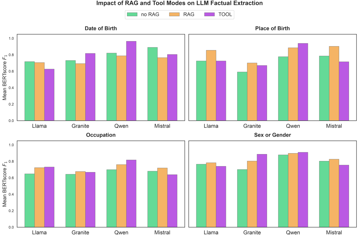
Figure 1: Mean BERTScore F_1 by models and modes for the four properties.
