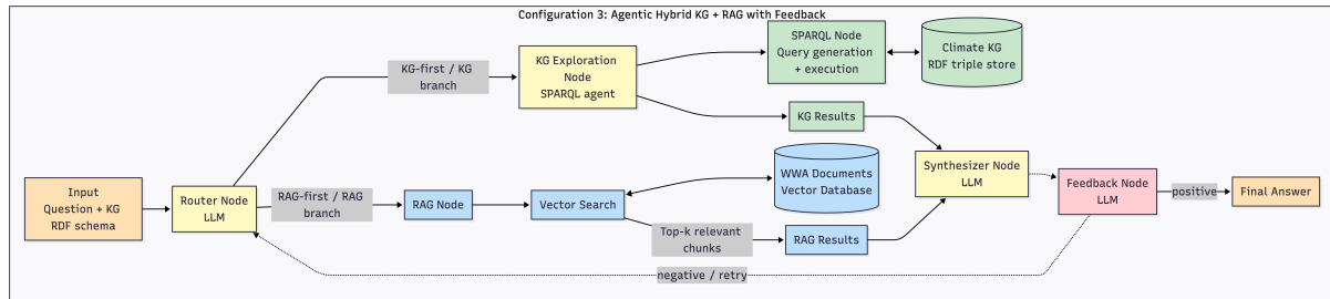
Figure 3: Visualization of the hybrid fully agentic type of configuration. The dotted arrow indicates an optional feedback loop that marks a distinction between two configurations, with and without the post-retrieval feedback.
