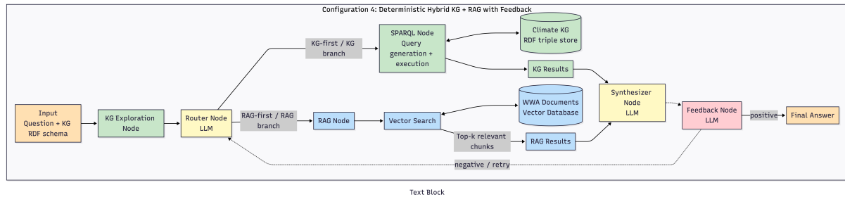
Figure 4: Visualization of the hybrid partially agentic (deterministic) type of configuration. The dotted arrow indicates an optional feedback loop that marks a distinction between two configurations, with and without the post-retrieval feedback.
