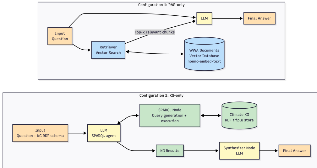
Figure 2: Visualization of the two base configurations: RAG-only in the top diagram and KG-only in the bottom diagram.
