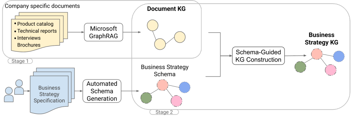
Figure 1: Overview of the proposed two-stage pipeline for constructing a Business Strategy Knowledge Graph from company documents and expert knowledge.
