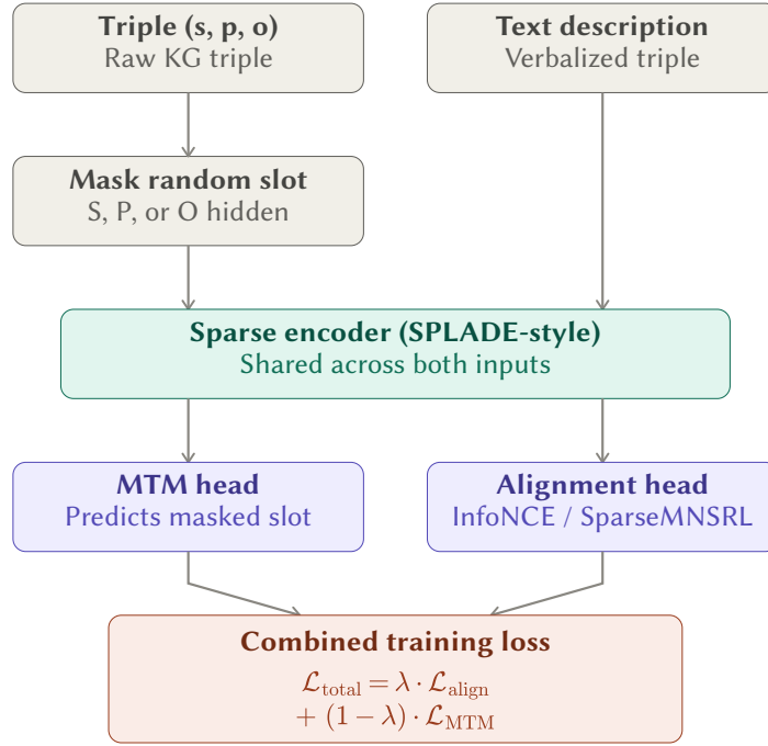
Figure 1: Overview of the MTM training pipeline. A triple and its verbalized text form are encoded by a shared sparse encoder (SPLADE-style); the triple branch is corrupted by masking one slot (subject, predicate, or object) before encoding. The resulting representations support two heads: an MTM head that reconstructs the masked slot, and an alignment head that scores text-triple correspondence via SparseMNSRL. The two objectives are combined into a single training loss, weighted by \lambda .
