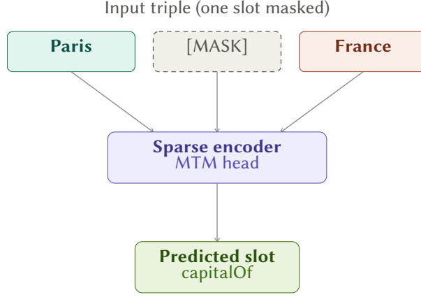
Figure 2: Masked Triple Modeling: one triple slot is masked (here, the predicate), and the sparse encoder’s MTM head predicts it from the remaining subject and object.
