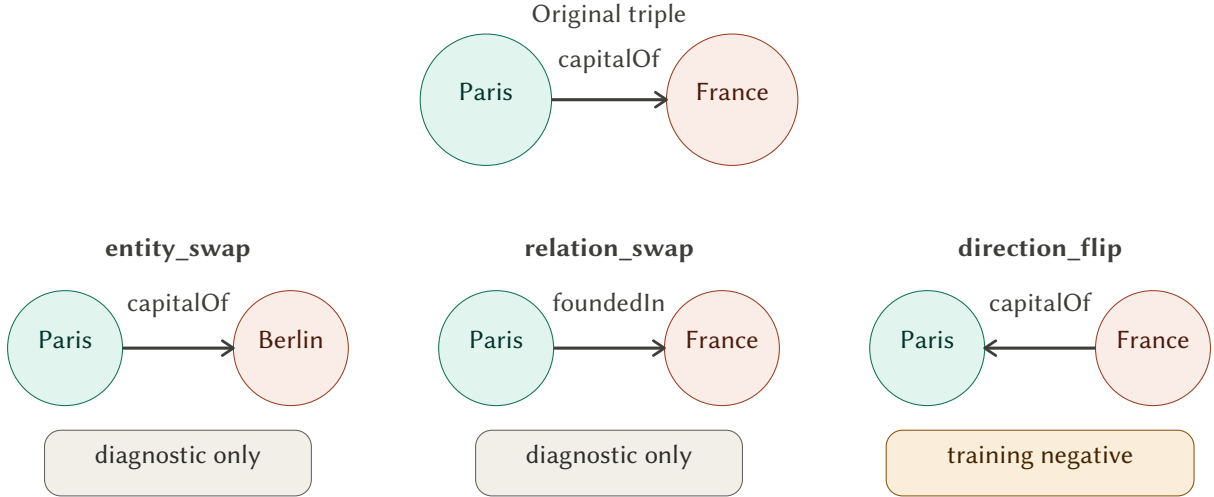
Figure 3: The three corruption types derived from a valid triple (Paris, capitalOf, France). Entity swap and relation swap are used exclusively in the directional-robustness diagnostic; direction flip is optionally used as a hard negative during training.
