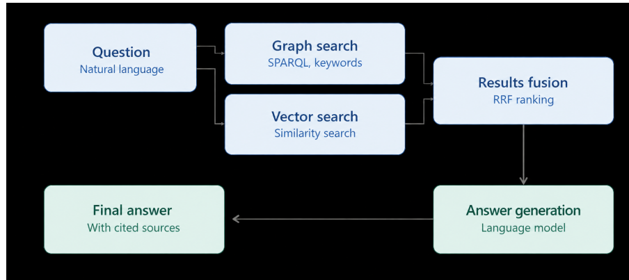
Figure 3: GraphRAG Pipeline
