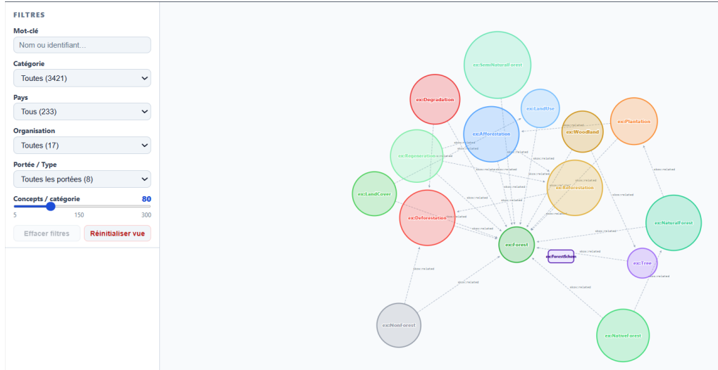
Figure 4: KG visualisation user interface
