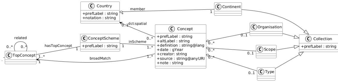
Figure 1: UML class diagram of the knowledge model for forest definitions
