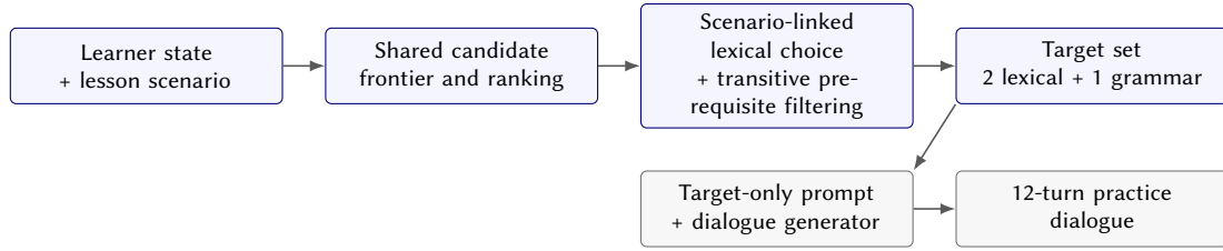
Figure 1: Curriculum-graph retrieval and generation pipeline. The generator receives target labels and a short grammar description, but no mastery values, graph paths, prerequisite nodes, or relation text.
