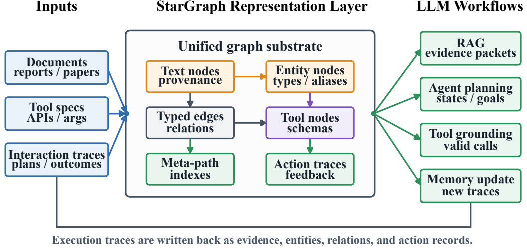
Figure 1: Overview of StarGraph as a shared substrate for RAG, agent planning, tool grounding, and memory updates.
