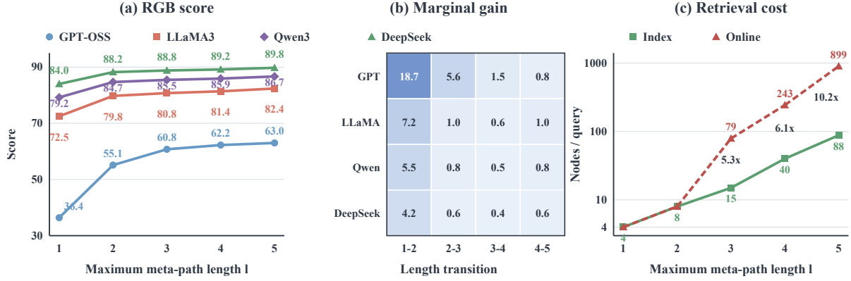
Figure 3: Meta-path sensitivity: (a) measured RGB scores across four backbones, (b) stepwise gains, and (c) retrieval cost.
