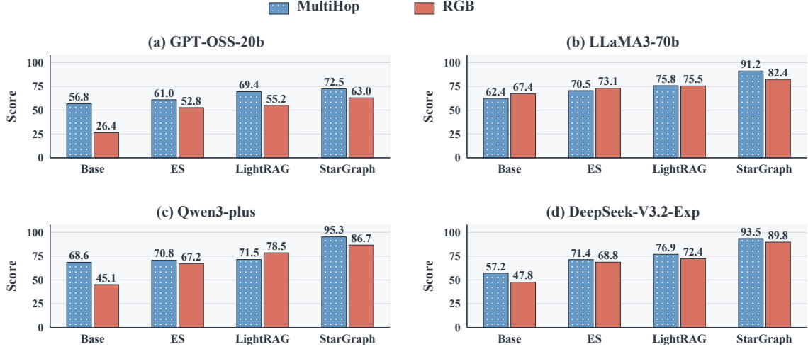
Figure 2: RAG-specific scores across four backbones. Each panel compares Base, ES, LightRAG, and StarGraph on MultiHop (blue) and RGB (orange).
