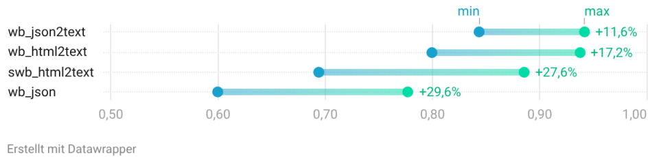
Figure 1: Range of MRR values across all evaluated retrieval configurations for each knowledge representation.
